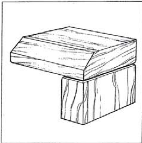
Group 4 - Veneer Top with 1/2" Wood Bevel Edge & Veneer End Panel with 1/4" Wood Eased Edge, 1 1/4" Thick
