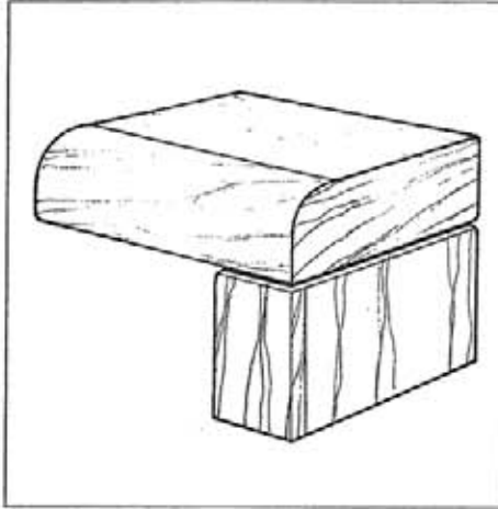
Group 3 - Laminate Top with 1/2" Wood Radius Edge & Laminate End Panel with 1/4" Wood Eased Edge, 1 1/4" Thick
