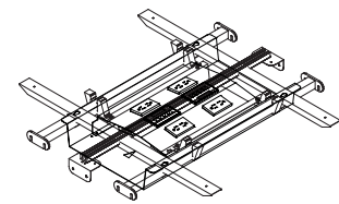
Support Structure
