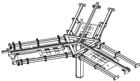
Support Structure
